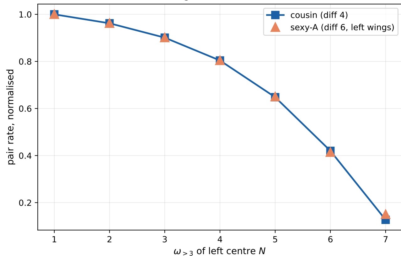
cousin \equiv sexy-A: identical \omega -curves (shared right member 6(N+1)-1 )
