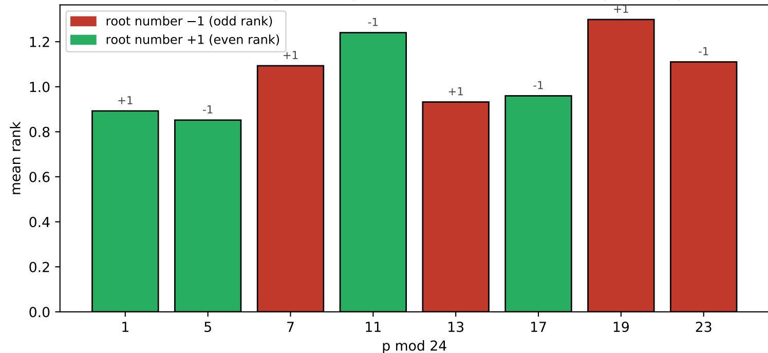
Mean rank is organized by root number (mod 24), not by 6N wing
