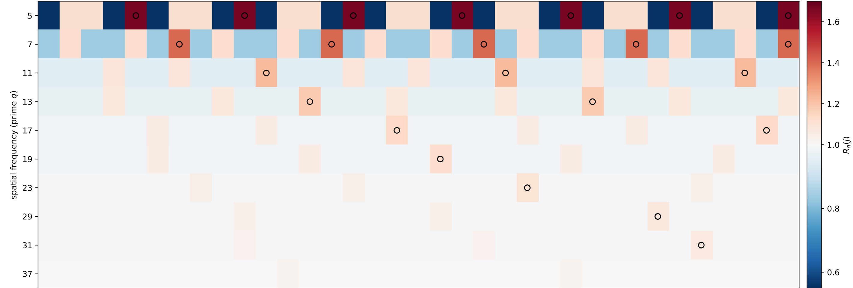
(A) single-frequency amplitude R_q(j) — State A (constructive) marked \circ ; amplitude fades as O(1/q^2) with q
