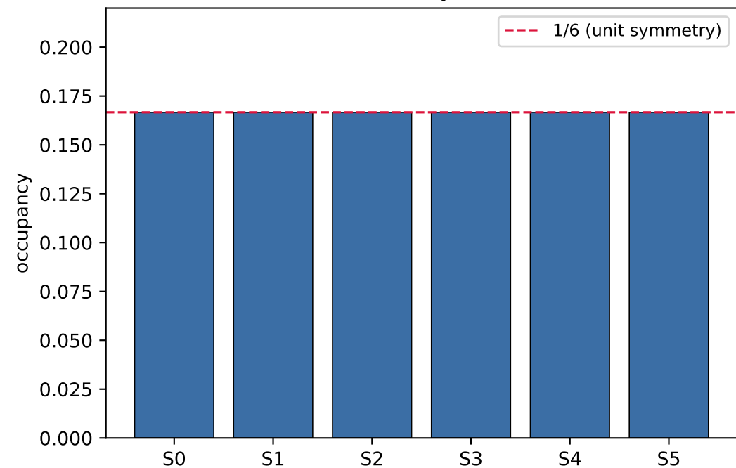
(A) Instrument gate: Eisenstein prime sextant occupancy ( N \leq 2.5 \times 10^5 ): exactly 1/6, maxdev = 0
