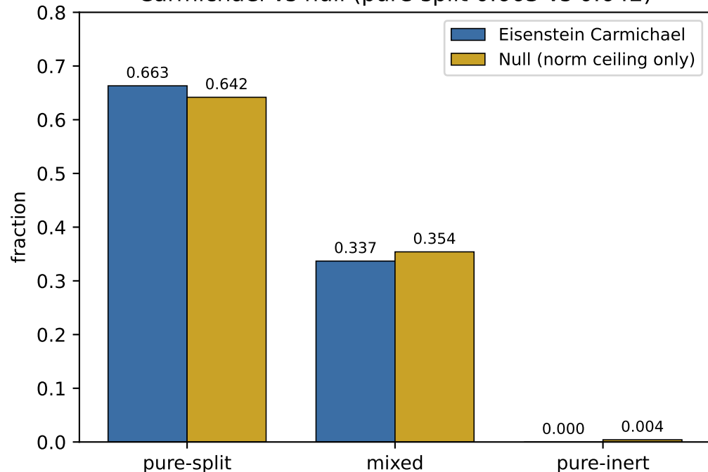
(B) Korselt colour-blindness: type spectrum Carmichael vs null (pure-split 0.663 vs 0.642)
