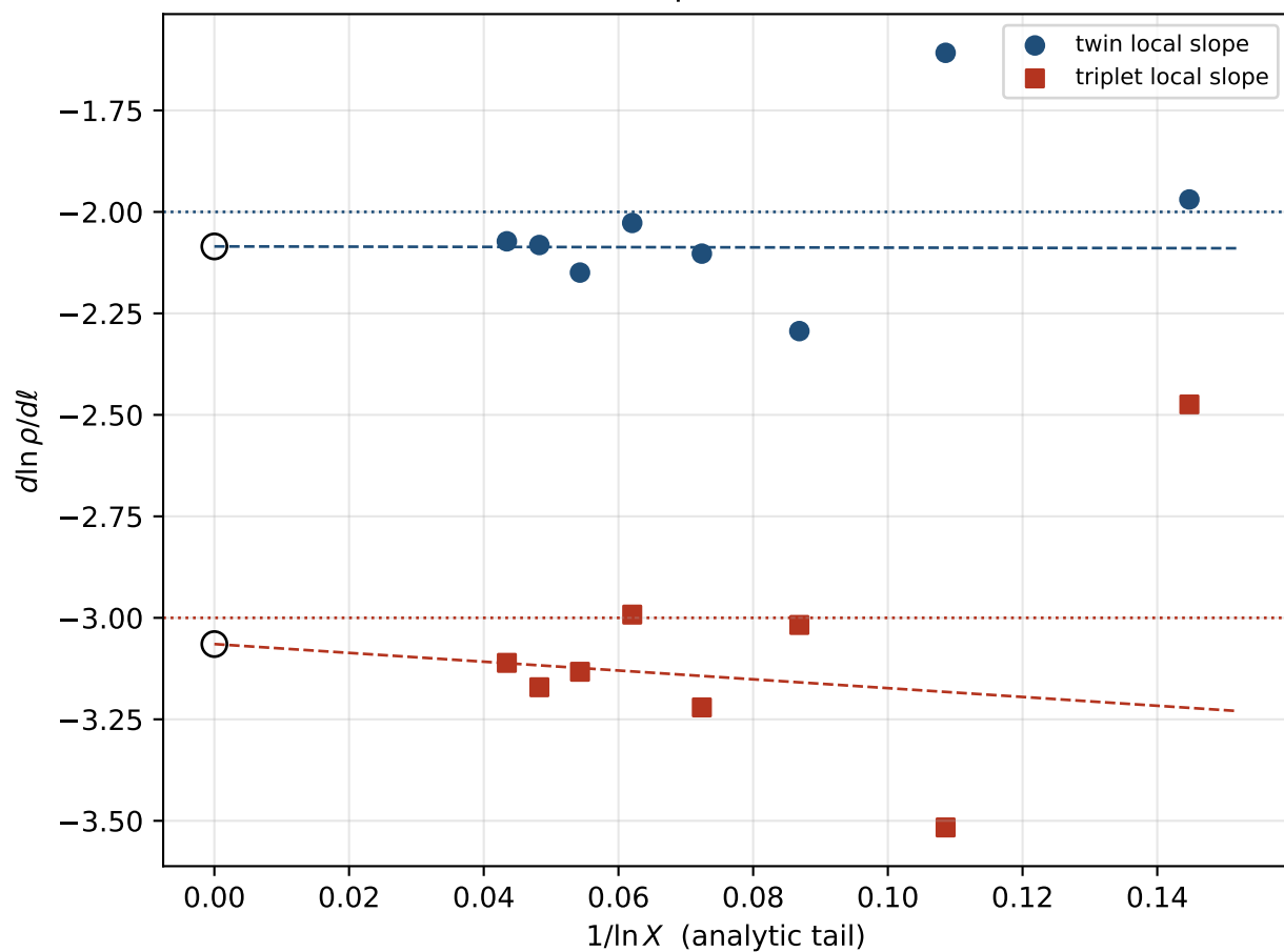
(C) tail dissolves: slope \rightarrow -2, -3 as 1/\ln X \rightarrow 0
