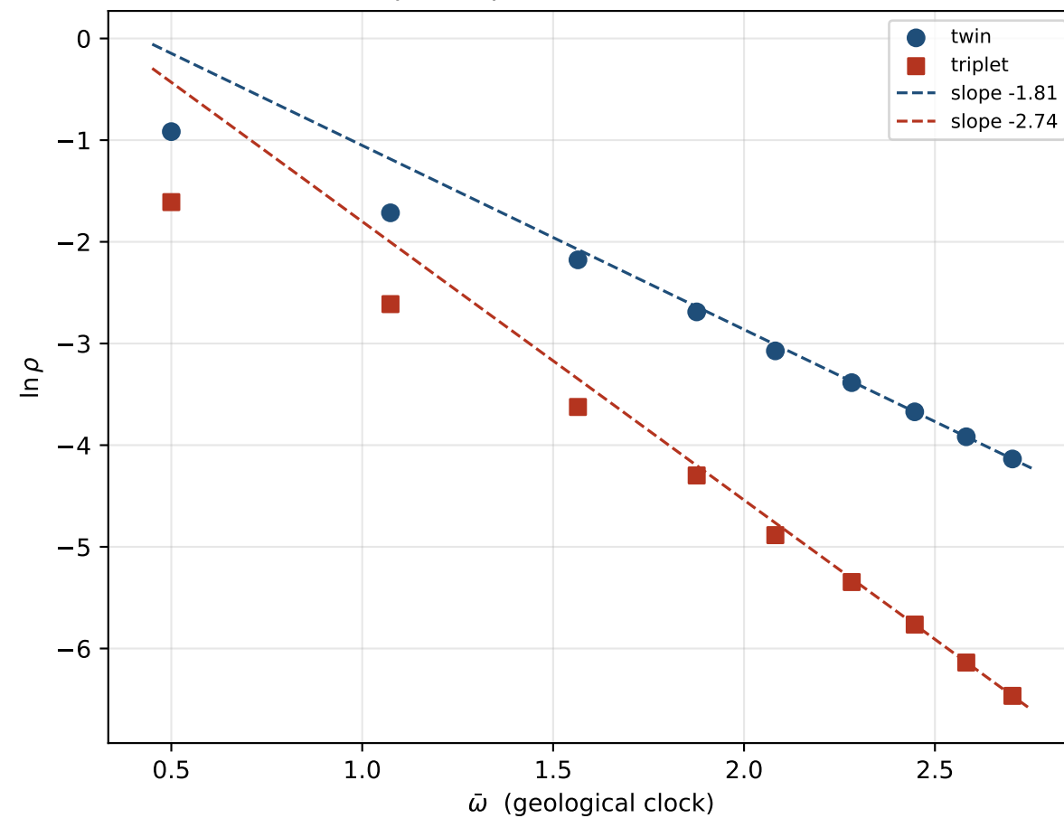
(B) \bar{\omega} phase plane: ratio = 1.51 (= 3/2)
