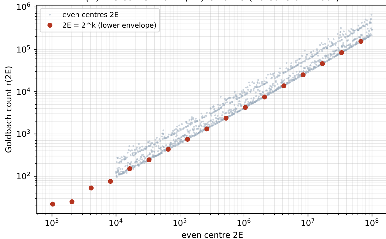
(A) the comet: raw r(2E) GROWS (no constant floor)
