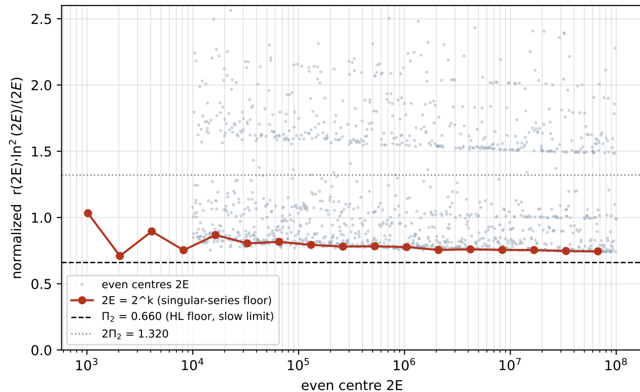
(B) normalized floor frozen > 0 (powers of 2), \rightarrow \Pi_2 slowly
