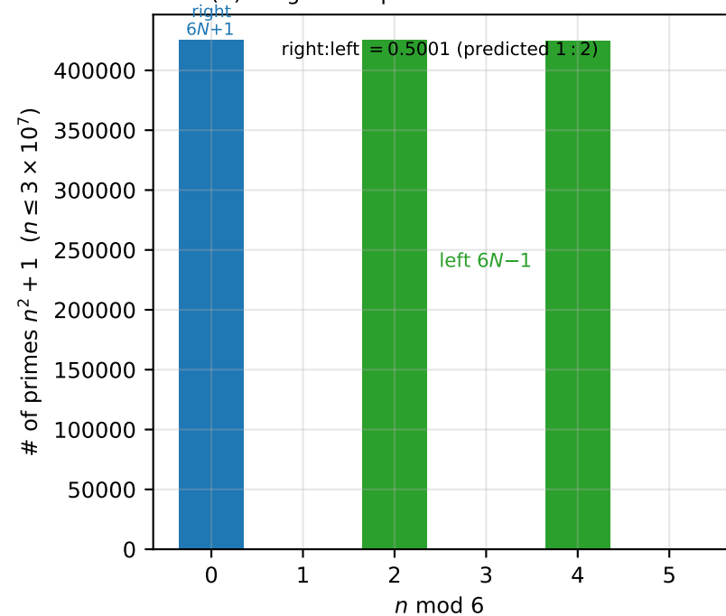
(A) wing decomposition: odd n annihilated
