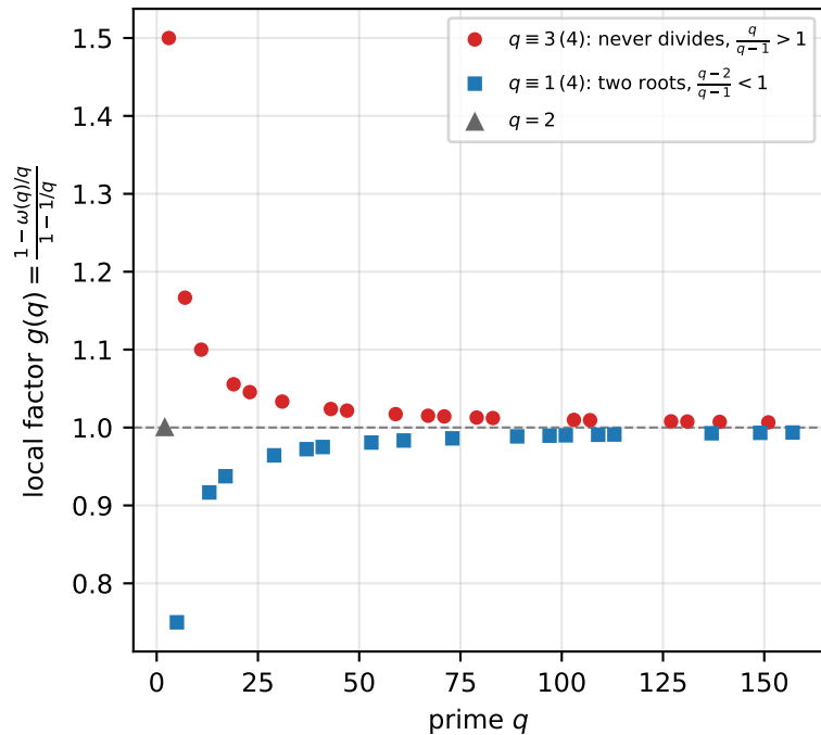
(B) the (-1|q) character spectrum
