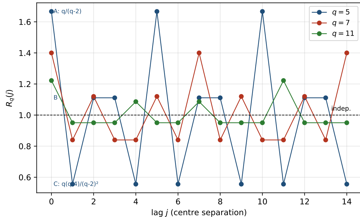
(B) three quantized states per prime ( A/B > 1 , C < 1 )
