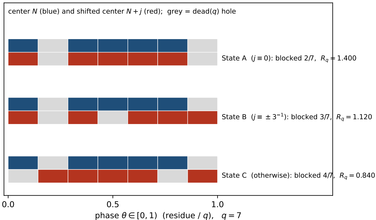
(A) two castellated bars on \mathbb{T}^1 ; overlap = joint survival
