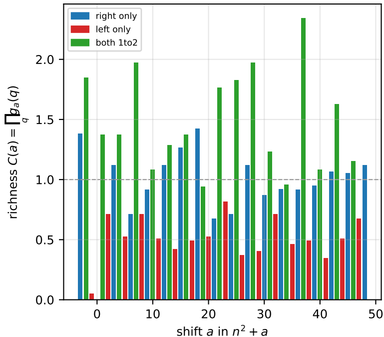
(A) the a -spectrum: mask (colour) \times richness
