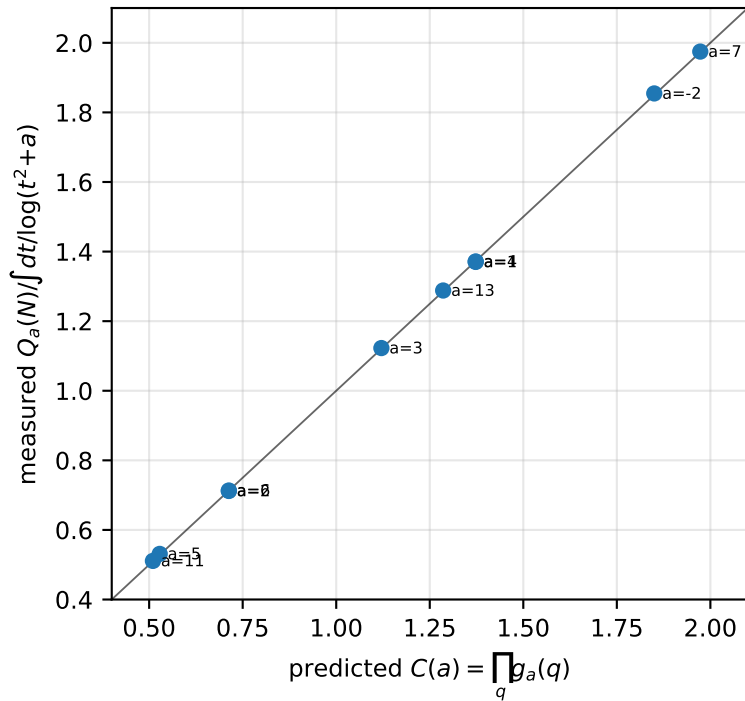
(B) Bateman--Horn holds across the family
