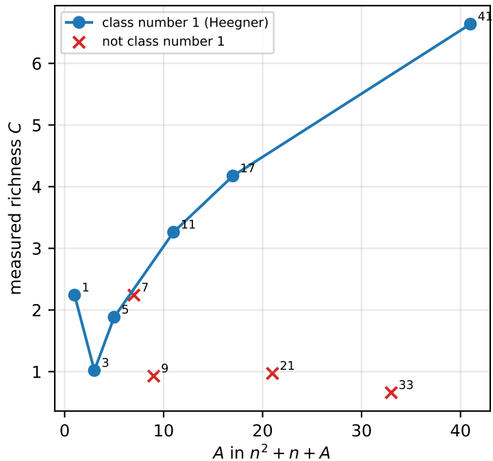
(B) the class-number-1 ladder, up to n^2 + n + 41
