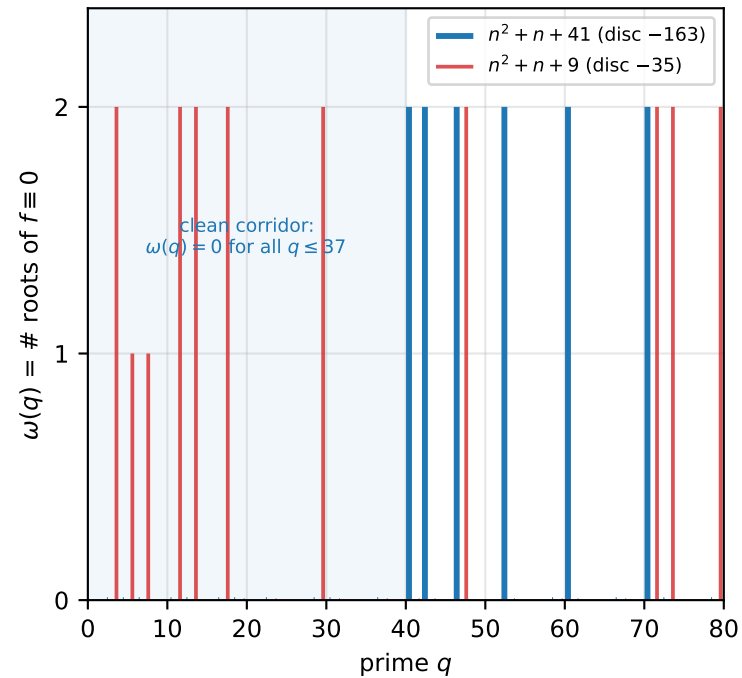
(A) the Heegner corridor of Euler's polynomial
