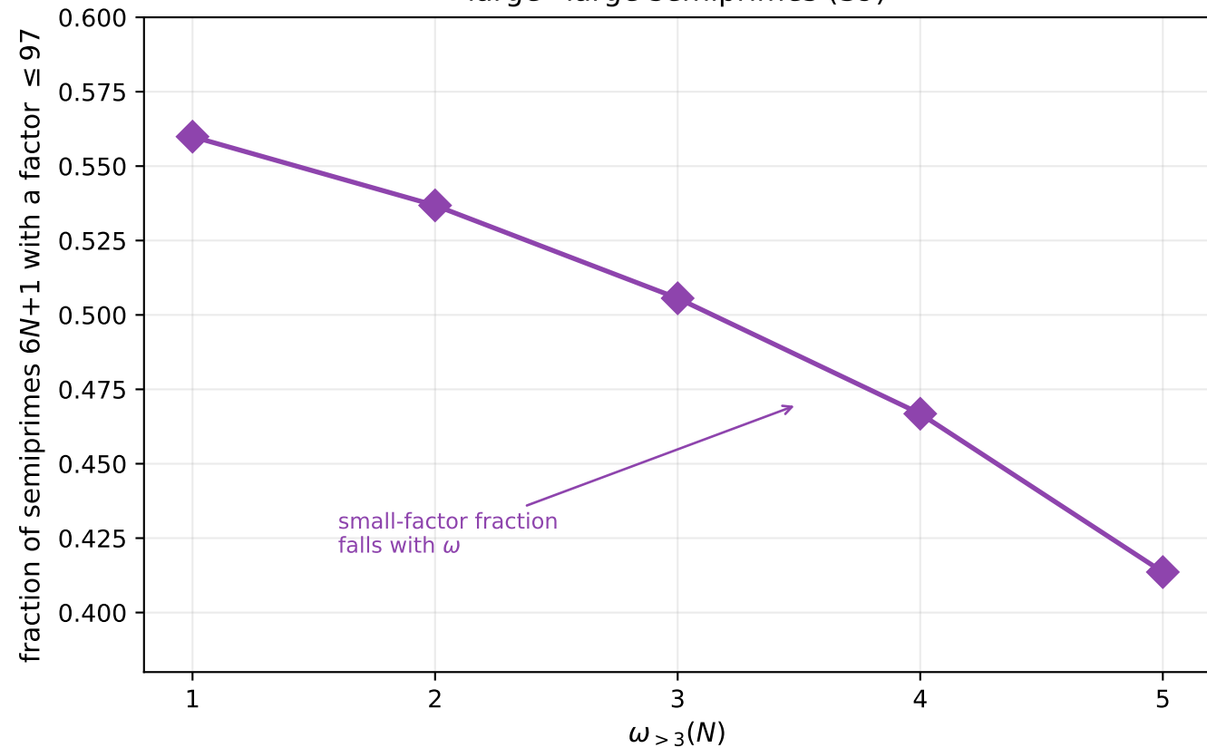
Mechanism: factor-rich N pushes 6N+1 toward large \times large semiprimes (S9)
