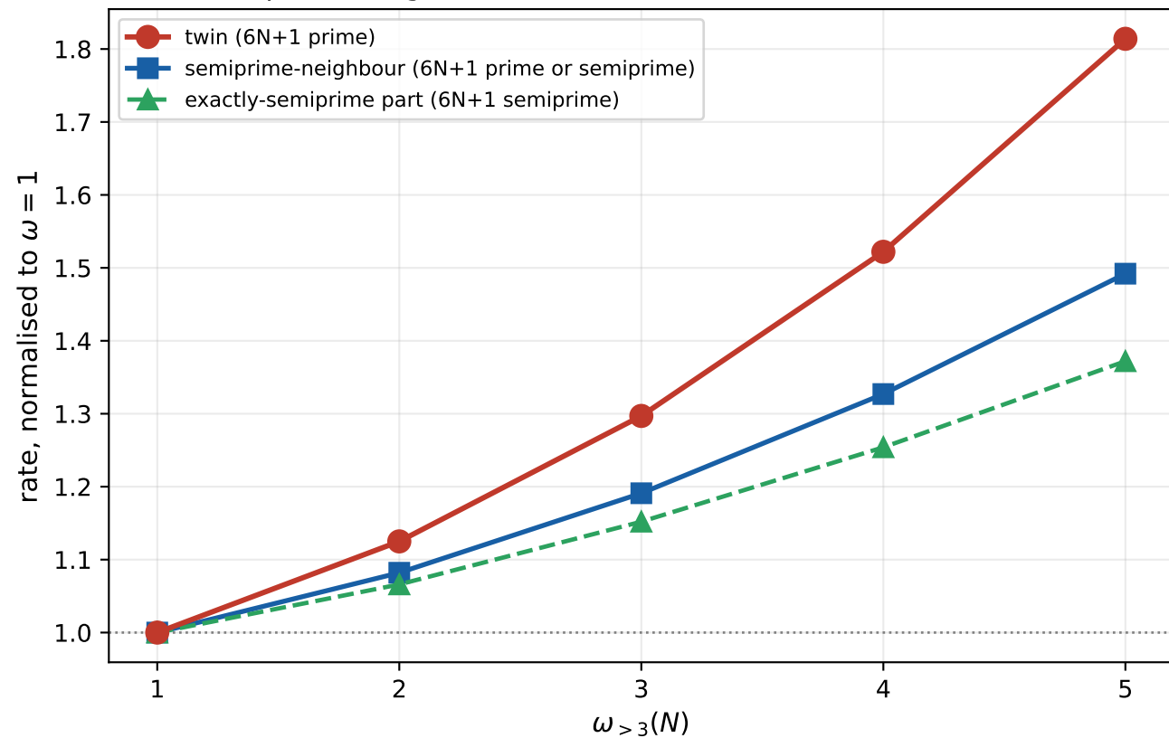
Semiprime-neighbour enrichment is slower than the twin (S9)
