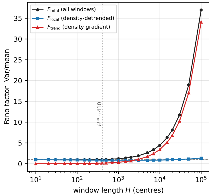
(A) variance decomposition
