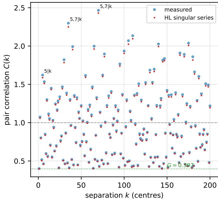
(B) local arithmetic: C(k) vs Hardy--Littlewood
