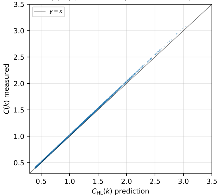
(A) C(k) : all k \leq 3000 (median dev. 1.7%)
