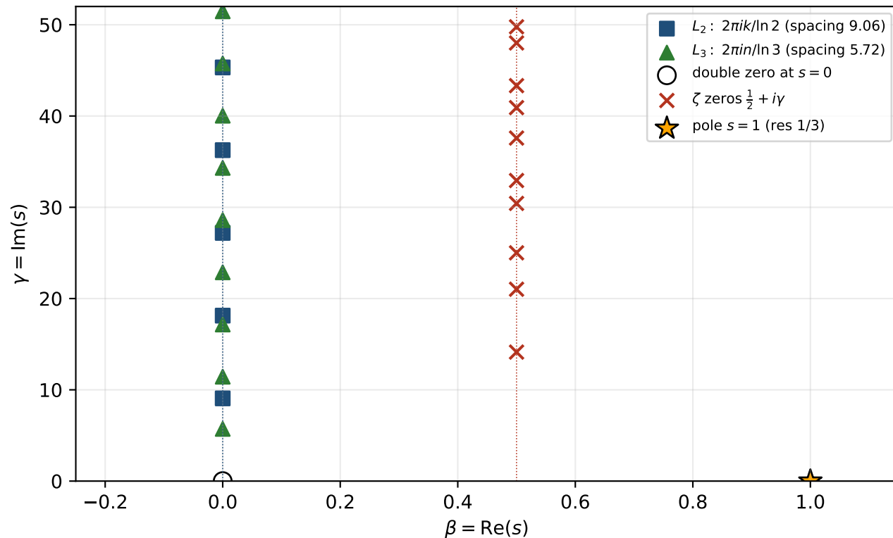
(A) zero map (upper half-plane)
