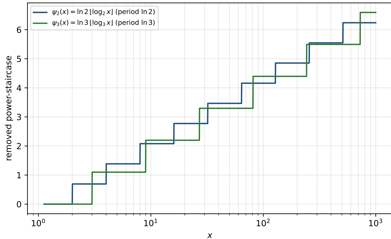
(B) the 2- and 3-power staircases stripped from \psi ; their Fourier modes = L_2, L_3
