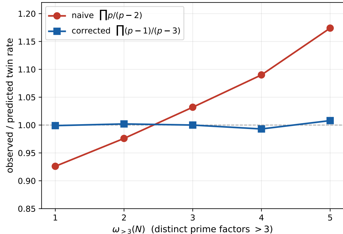
Factor-resolved test of the local model (shell S8, \sim 10^8 nodes)
