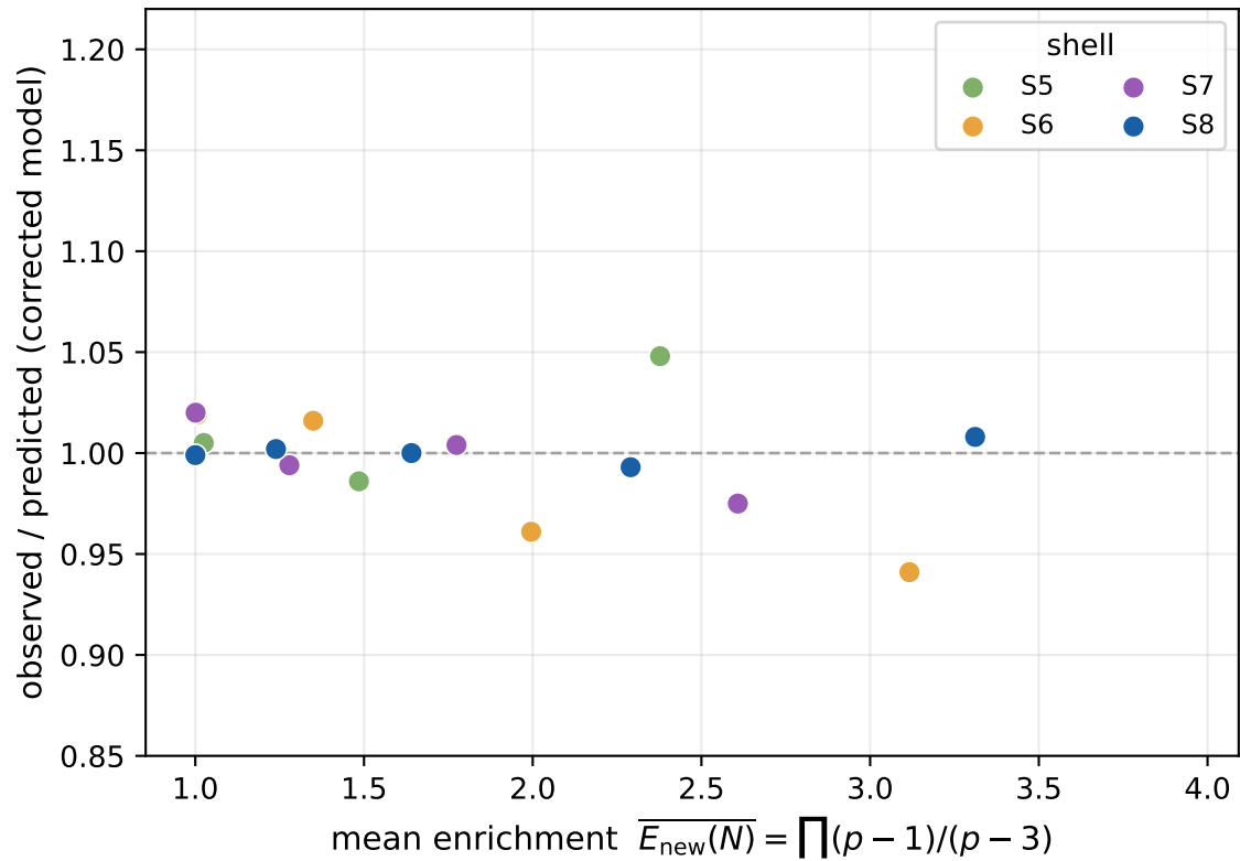
Corrected model holds across shells &amp; enrichment range
