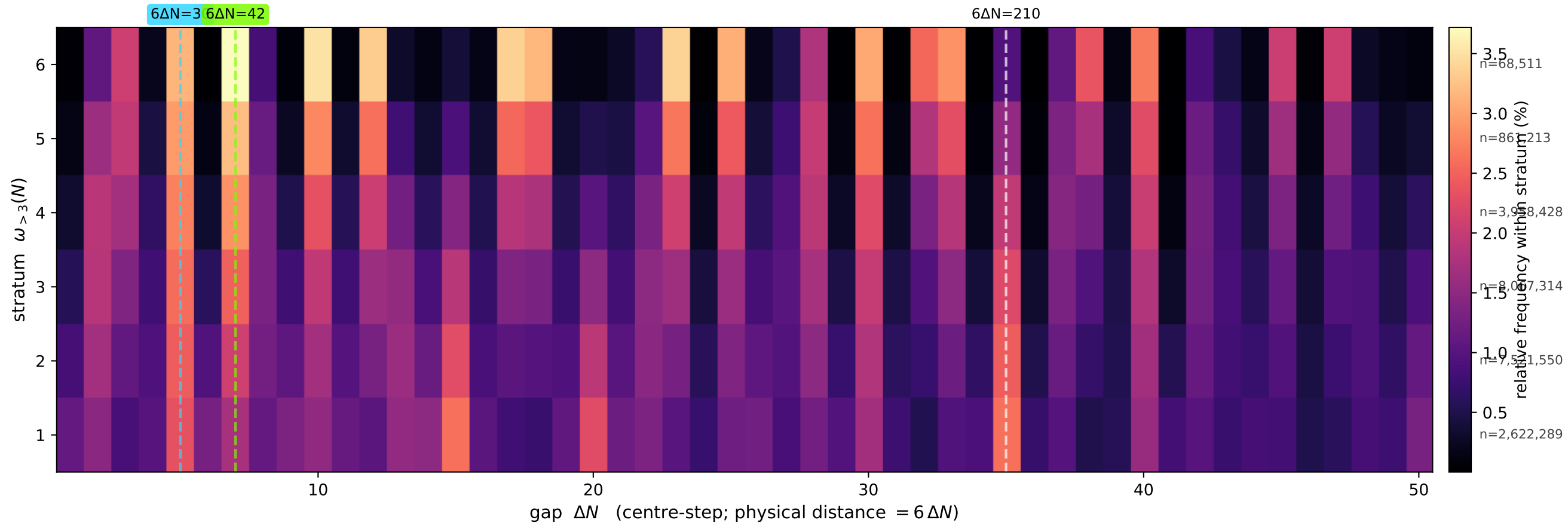
Twin-prime gap distribution by \omega_{>3} in S_{10} (strata with \geq 10^4 gaps; \omega \geq 7 omitted: insufficient sample)
