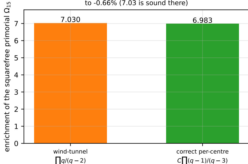
(B) for the primordial centre the two agree to -0.66% (7.03 is sound there)
