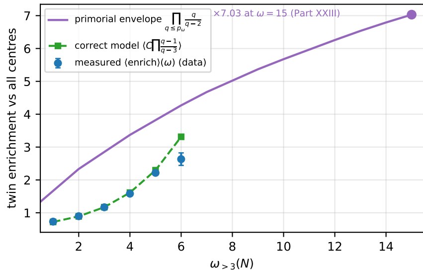
(A) the wind-tunnel tilt: data sits far below the primordial envelope at matched \omega
