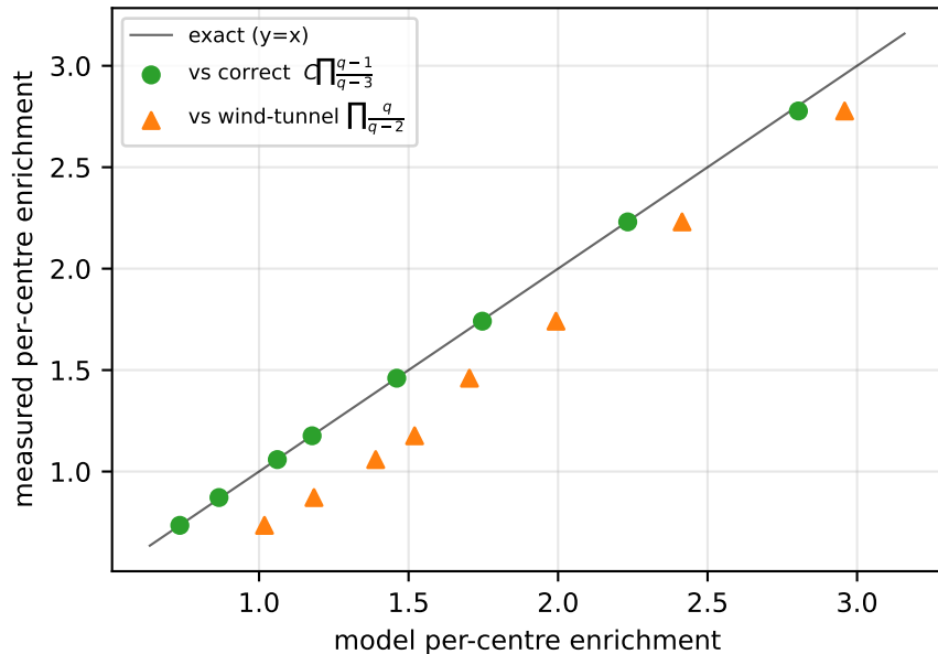
(B) per-centre: wind-tunnel M overshoots; C=0.7216
