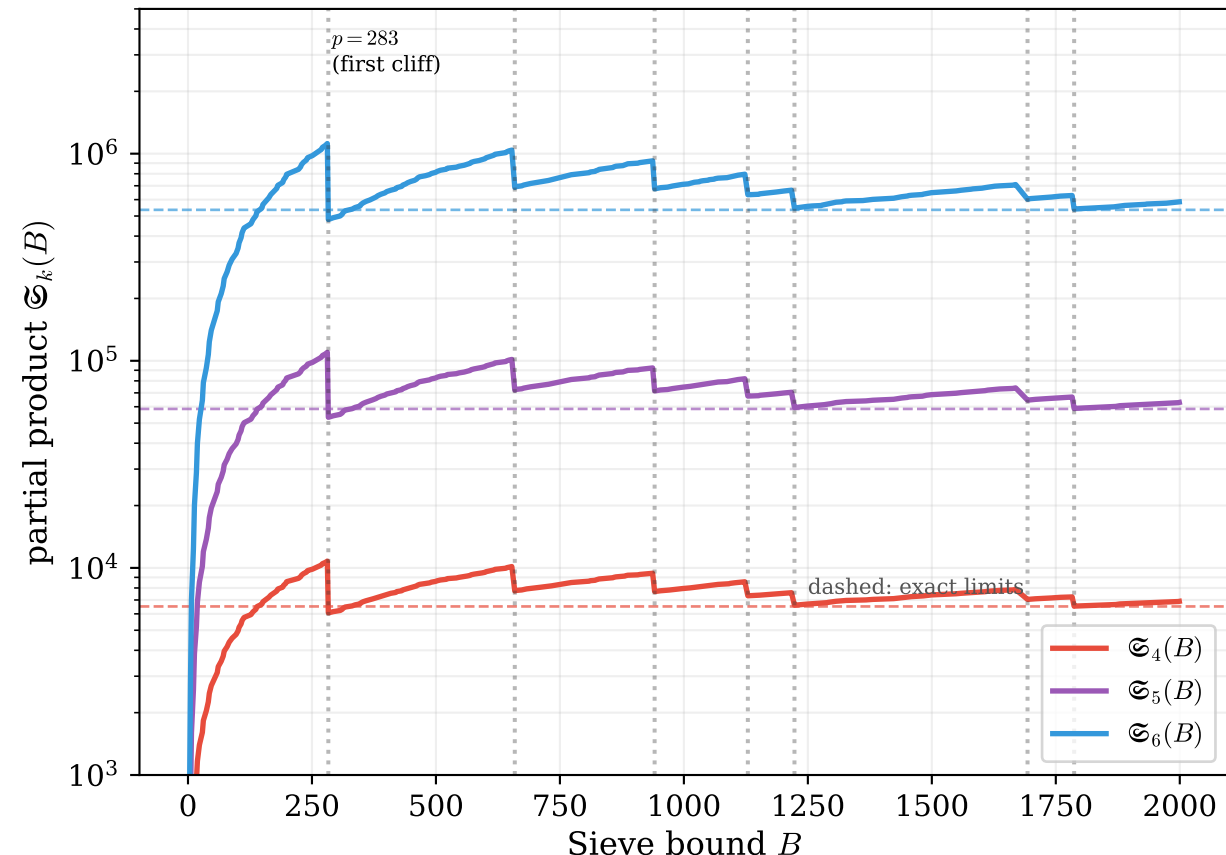
(b) Euler product with the periodic obstruction
