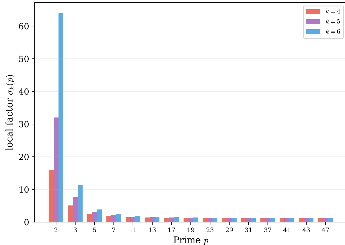
(a) Local factors, p < 50 (all non-resonant, \omega_k = 0 )
