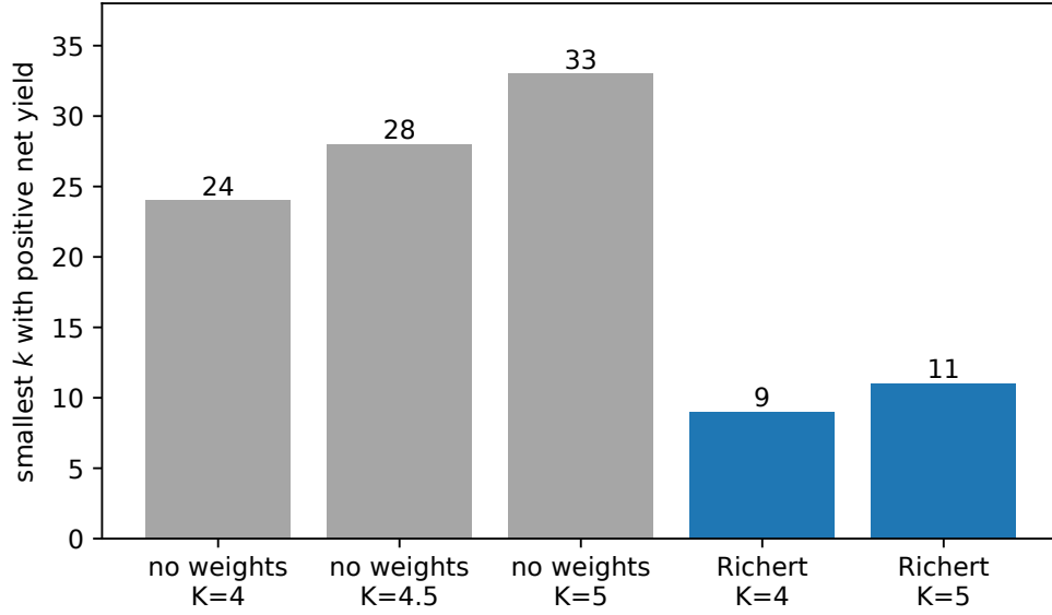
FIGURE 2. Smallest bound k for \Omega(N-p) obtained by floating-point parameter scans, without weights and with Richert's weights, for several values of the switching constant K . Only the value k = 9 ( K = 4 , Richert's weights) is certified (Lemma 5.1); the other values are illustrative.
