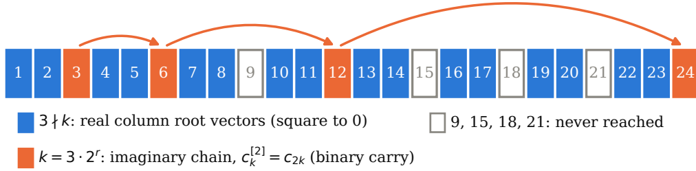
FIGURE 2. (a) The first non-injective degree k_m of R_{\sigma F} on u_m (dots, computed for m \leq 14 ; k_{15} \leq 95 ) against d(m) of Theorem C (steps) and the naive guess m(m-1)/2 (dashed). (b) The mechanism: the column subalgebra generated by c_1, c_2, c_3 contains c_k for 3 \nmid k and the imaginary chain c_3 \rightarrow c_6 \rightarrow c_{12} \rightarrow c_{24} produced by the 2-map (a binary carry), but never c_9, c_{15}, c_{18}, c_{21}, \dots ; the staircase \omega = \prod_{k \in \mathcal{H}_m} c_k has degree d(m) and is annihilated by \sigma F (Theorem 5.3).
