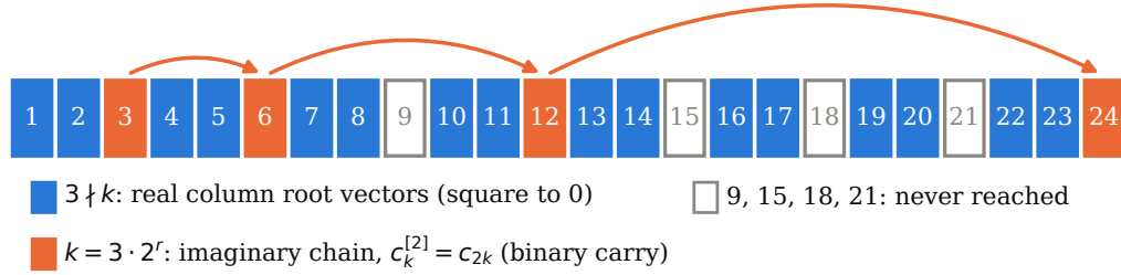
FIGURE 2. (a) The first non-injective degree k_m of R_{\sigma F} on u_m (dots, computed for m \leq 12 ) against d(m) of Theorem C (steps) and the naive guess m(m-1)/2 (dashed). (b) The mechanism: the column subalgebra generated by c_1, c_2, c_3 contains c_k for 3 \nmid k and the imaginary chain c_3 \rightarrow c_6 \rightarrow c_{12} \rightarrow c_{24} produced by the 2-map (a binary carry), but never c_9, c_{15}, c_{18}, c_{21}, \dots ; the staircase \omega = \prod_{k \in \mathcal{H}_m} c_k has degree d(m) and is annihilated by \sigma F (Theorem 5.3).
