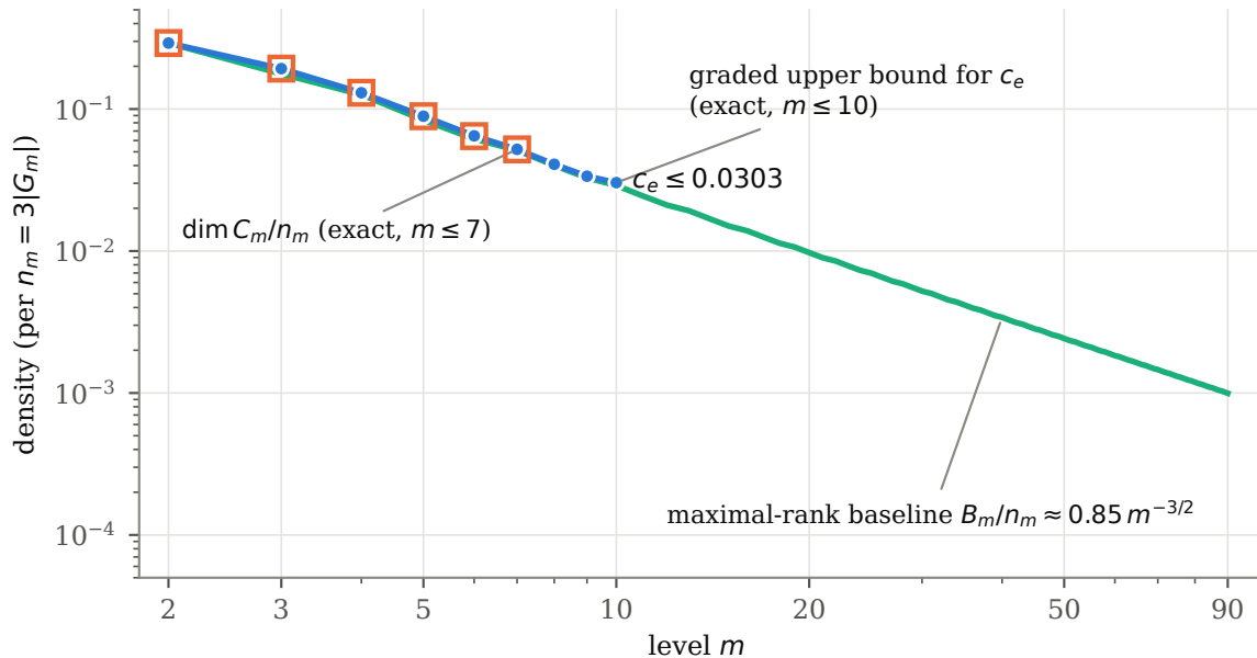
Upper bounds for the cokernel density c_e
