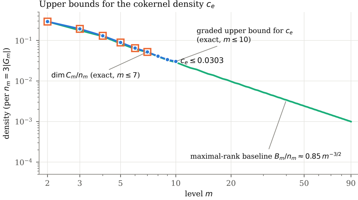
FIGURE 1. Upper bounds for c_e (log-log). Squares: exact \dim C_m/n_m ( m \leq 7 ). Dots: the graded upper bound \dim \text{coker}(R_{\sigma_F}|u_m)/n_m (Lemma 2.4), exact for m \leq 10 , giving c_e \leq 0.0303 . Line: the maximal-rank baseline B_m/n_m (Section 8), computed exactly for m \leq 90 ; the graded bound equals the baseline plus the excess e_m/3 , and c_e = 0 is equivalent (at the graded level) to e_m \rightarrow 0 .
