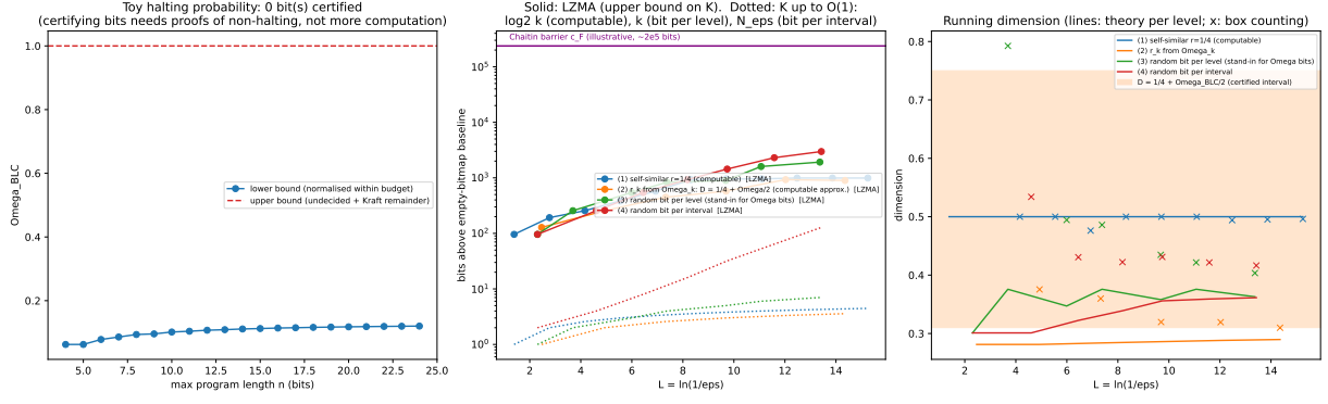
Figure 1: Left: lower bound on the toy halting probability \Omega_{BLC} against the maximal program length; the upper bound is trivial (see text). Middle: LZMA-compressed size above the empty-bitmap baseline (solid) and the complexity predicted by Propositions 3.1–3.3 up to O(1) (dotted) for the four constructions; the horizontal line marks the illustrative Chaitin scale c_F . Right: running dimension per stage (lines) and box-counting estimates (crosses); the band is the interval for \frac{1}{4} + \frac{1}{2}\Omega_{BLC} implied by the bounds on \Omega_{BLC} .
