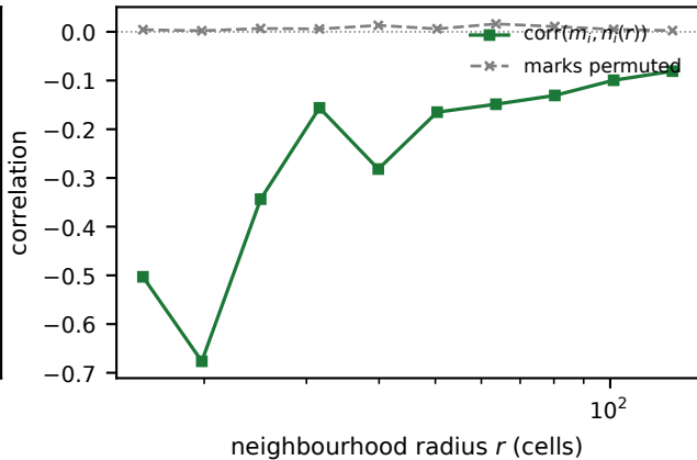
(b) does a domain's mass know its crowding?
