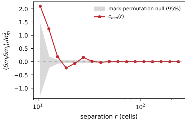
(a) do neighbouring domains have similar masses?
