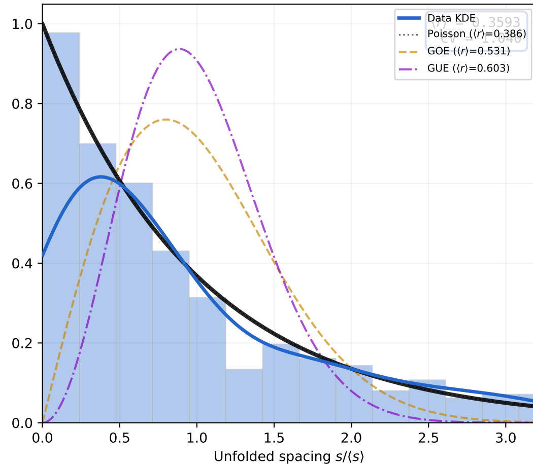
(c) Mixed Independent Clades (12 clades superposed, n=471 )
