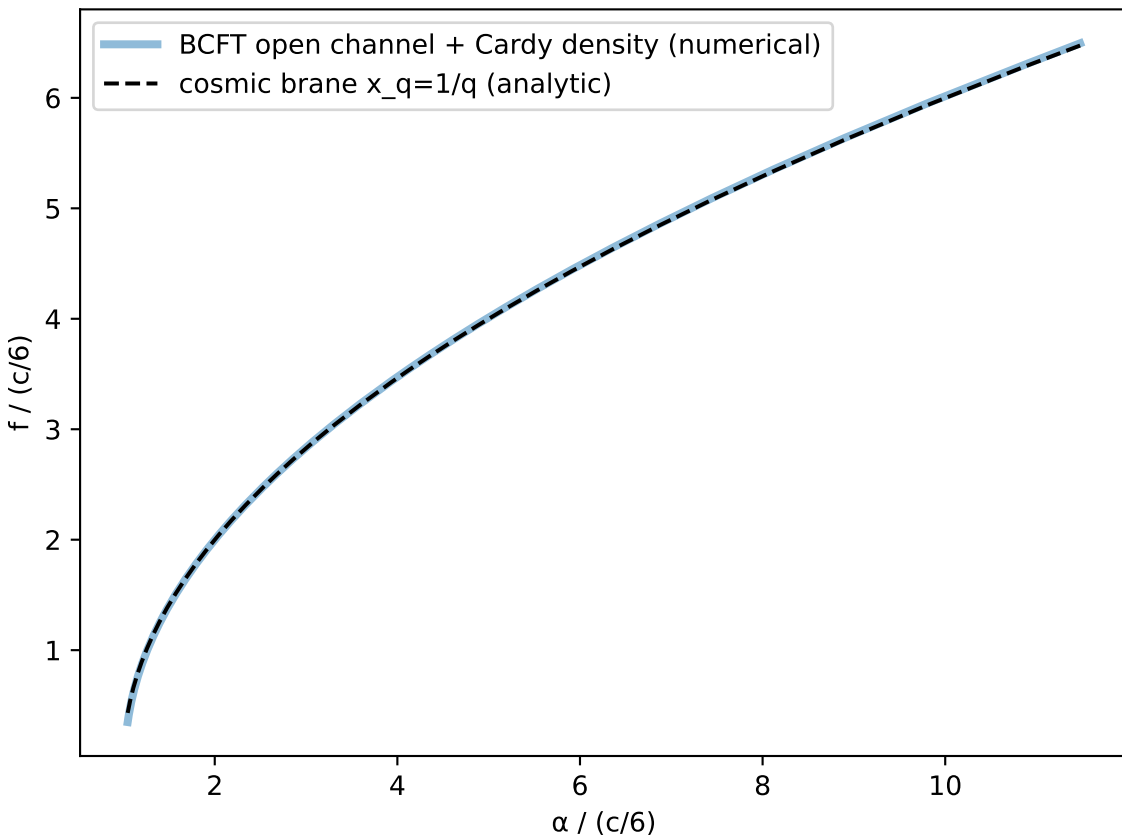
d=2 check: Schmidt spectrum = holographic singularity spectrum
