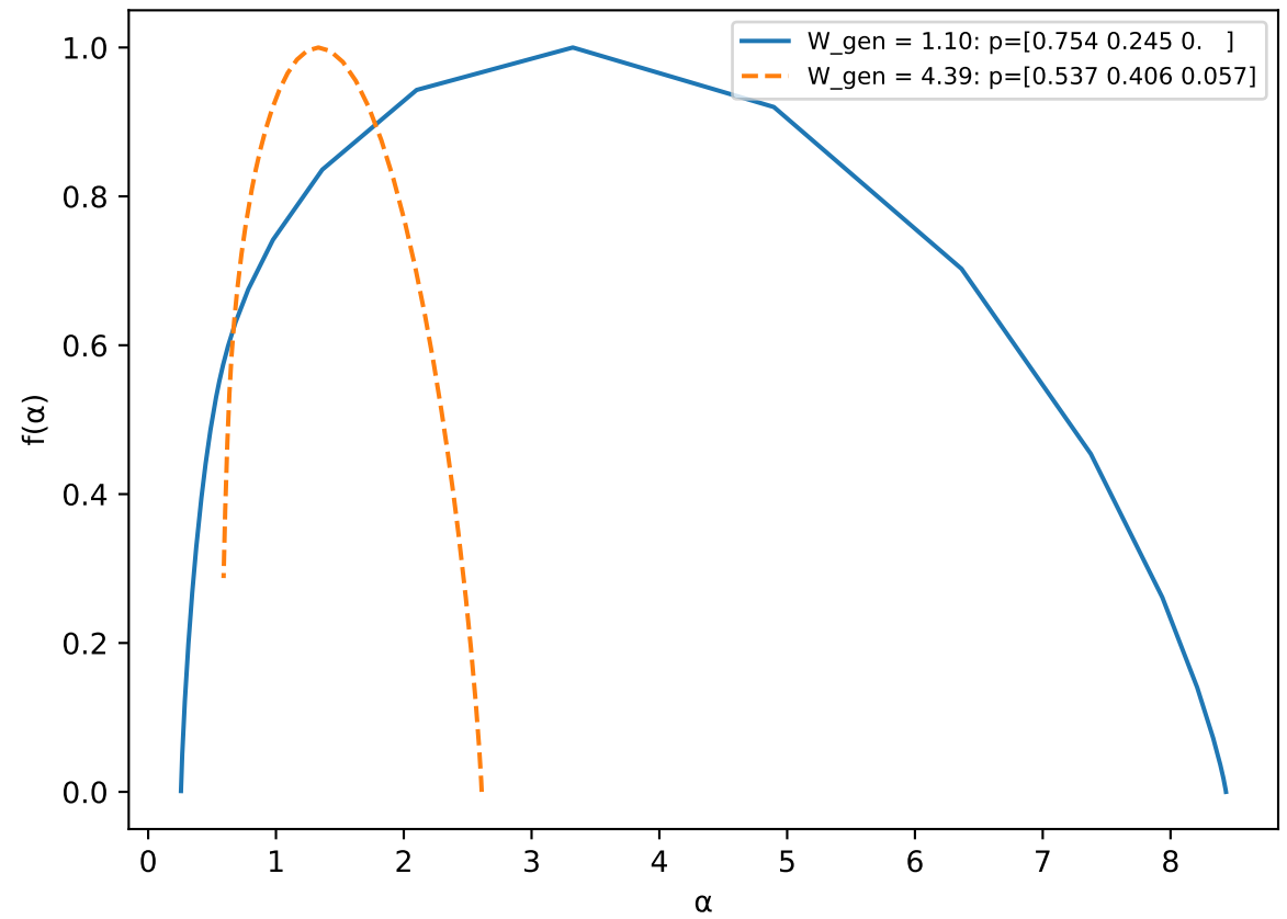
Sparse spectrum (Ising boundary operators) -> non-trivial multifracta
