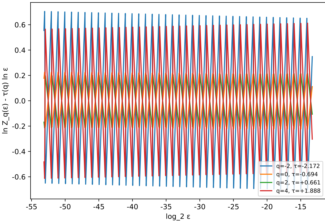
Lattice r=(1/2,1/4) : period \ln 2 for all q
