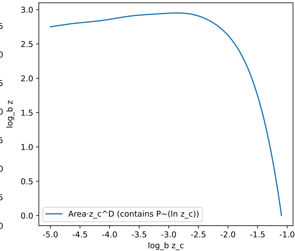
Log-periodic modulation of the bare area
