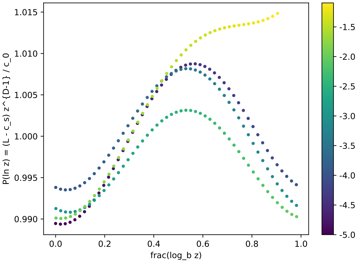
Log-periodic function P: periods folded onto each other
