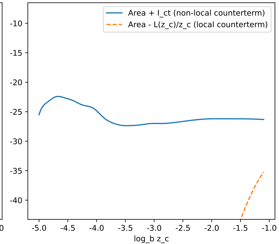
Renormalised entropy (units R^2/4G )
