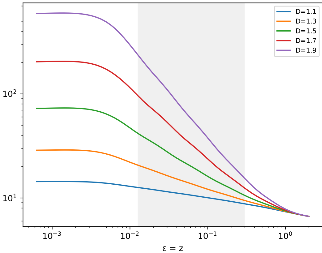
Cross-section length L(z) ( \sim z^{\{1-D\}} )
