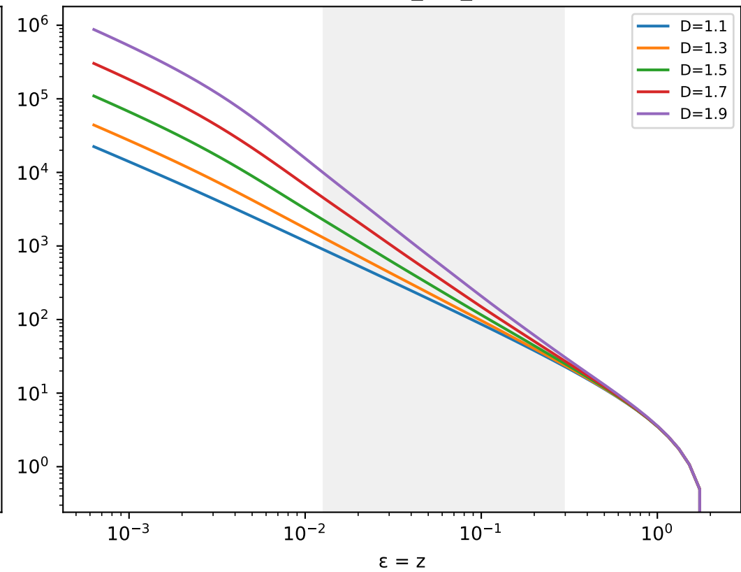
RT area \text{Area}(\epsilon) \sim 4G_N S_A ( \sim \epsilon^{\{-D\}} )
