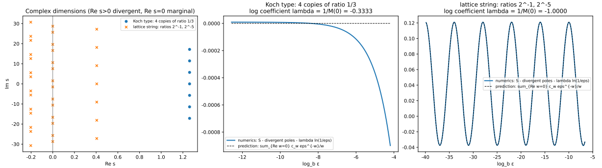
Figure 3: Left: complex dimensions of the Koch-type system and the (2^{-1}, 2^{-5}) lattice string. Middle and right: renormalised entropy after subtracting divergent poles and the logarithm (solid) against the prediction from marginal complex dimensions (dashed).
