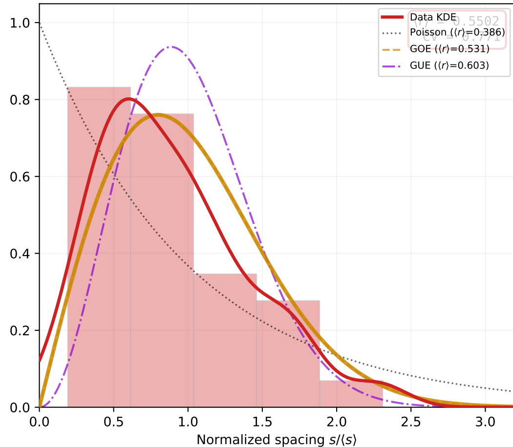
(c) N. Atlantic IRD Events (single source, n=34 , millennia)
