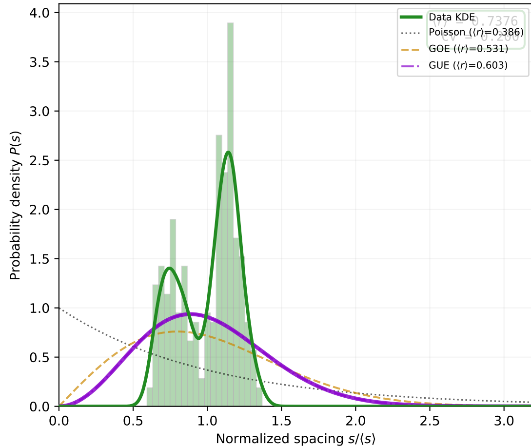
(a) Old Faithful Geyser (single source, n=271 , minutes)
