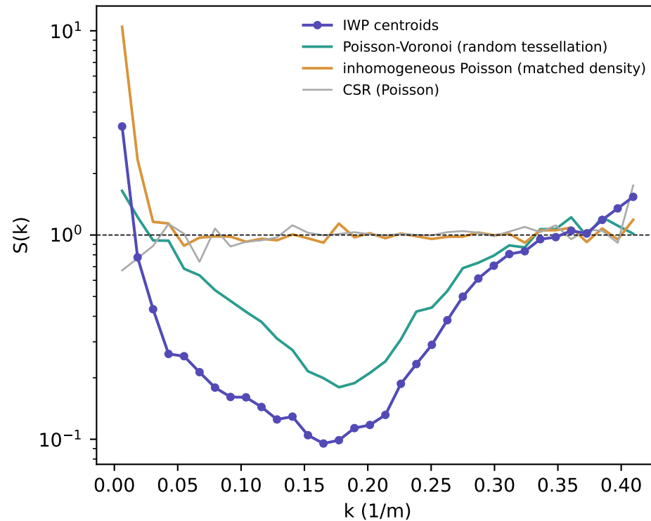
(b) structure factor: deep genuine dip, below random tessellation (c) number variance: long-range NOT hyperuniform
