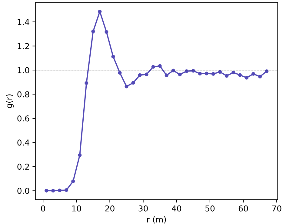
(a) pair correlation: hard-core + spacing \sim 17 m
