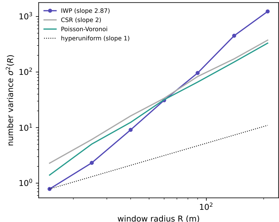
(b) structure factor: deep genuine dip, below random tessellation (c) number variance: long-range NOT hyperuniform
