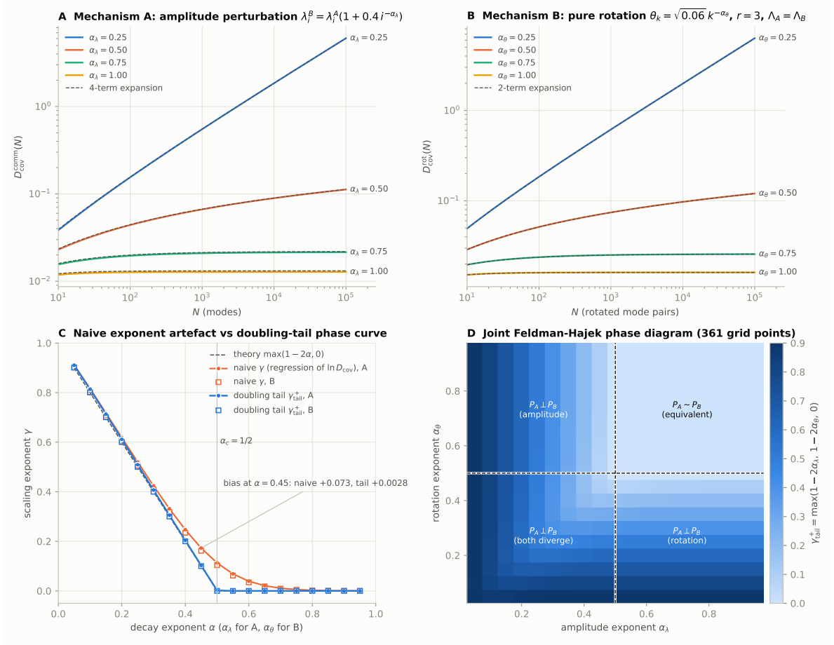
FIGURE 1. Spectral Kakutani criticality of covariance perturbations decaying along the mode index (file fig03 in figures/ ). A. Mechanism A: D_{comm}(N) on doubly logarithmic axes for \alpha_\lambda \in \{0.25, 0.5, 0.75, 1\} with the four-term expansion (2.3) summed (dashed) superposed: power-law divergence, logarithmic divergence, saturation at D_\infty(0.75) = 0.02157 and D_\infty(1) = 0.01278 . B. Mechanism B: D_{rot}(N) for the same exponents with the two-term expansion (2.6): the same three regimes, with saturation at 0.02577 and 0.01613, although every eigenvalue is unchanged. C. The naive exponent (orange) is a smooth curve through \alpha_c = 0.1729 (A) and 0.1619 (B) at \alpha = 0.45 , 0.113 and 0.104 at \alpha = \frac{1}{2} —while the doubling-tail exponent \gamma_{tail}^+ (blue) is the sharp kink \max(1 - 2\alpha, 0) of Theorem 4.1; filled circles are Mechanism A, open squares Mechanism B, and at \alpha = 0.45 the two estimators differ by +0.073 against +0.0028 (A). D. The joint phase diagram of Theorem 5.1: measured \gamma_{tail}^+ on the 19 \times 19 grid, with the boundaries \alpha_\lambda = \frac{1}{2} and \alpha_\theta = \frac{1}{2} (dashed). The lower-right quadrant is the rotation-driven singular phase of cryptic iso-spectral allostery; the upper-right quadrant is the only equivalent phase.
