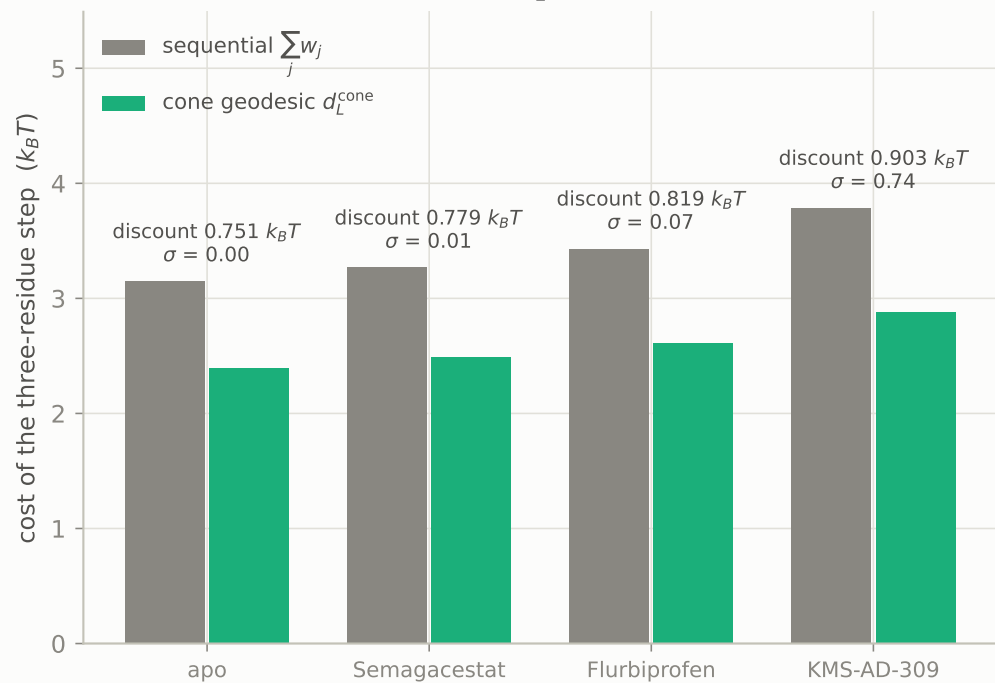
C Cone geodesic on \{0, 1\}^3 : d_L^{\text{cone}} = 2.284457 w < 3w
