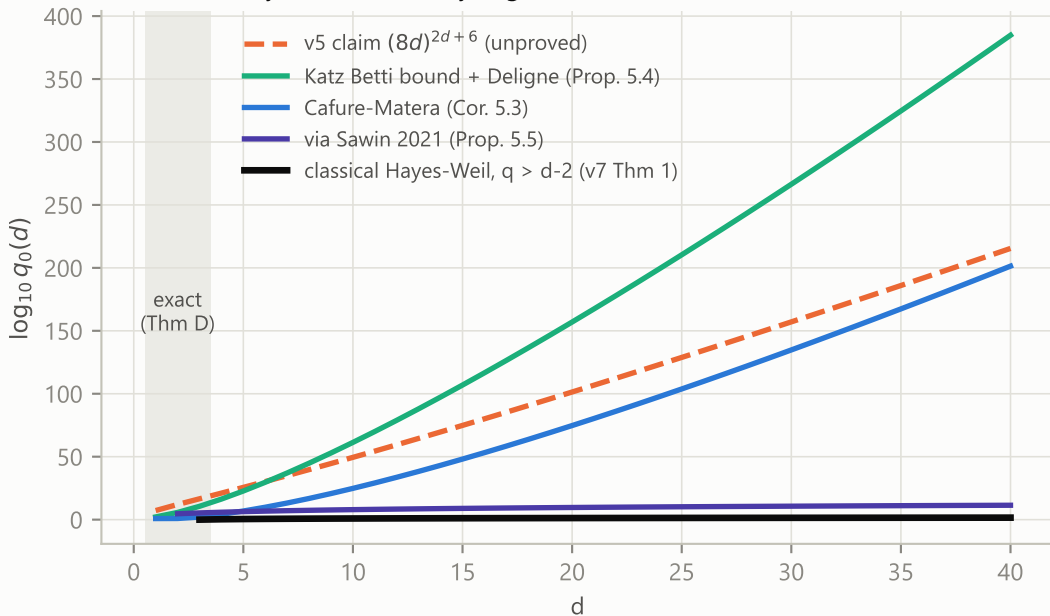
Thresholds beyond which every Legendre interval contains an irreducible
