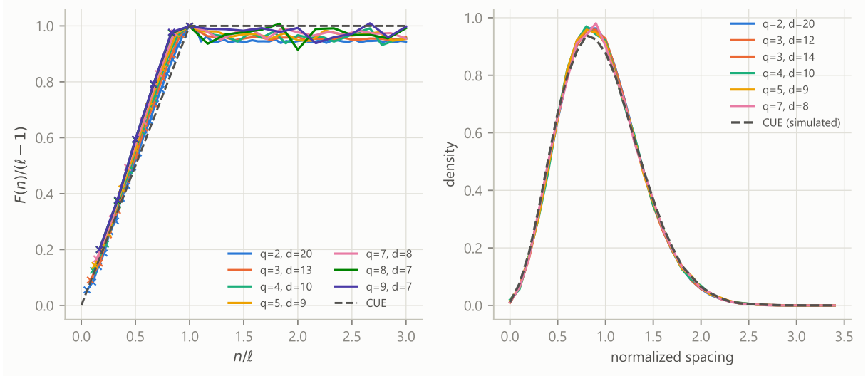
Figure 3: Left: the form factor F(n)/(\ell-1) against n/\ell for several (q, d) , with the CUE value \min(n, \ell-1)/(\ell-1) and the exact diagonal of Proposition 7.2 (crosses). Right: nearest-neighbour spacing densities against CUE.
