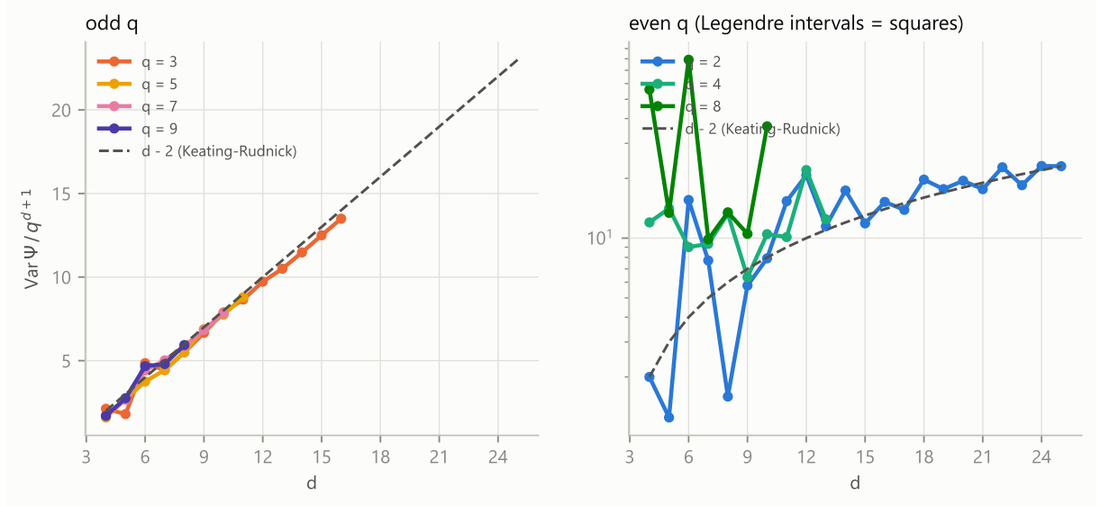
Figure 1: \text{Var}_f \Psi(f)/q^{d+1} (mean square deviation from q^{d+1} ) over all Legendre intervals. Left: odd q , against the Keating–Rudnick limit d - 2 . Right: even q , where the prediction fails.
