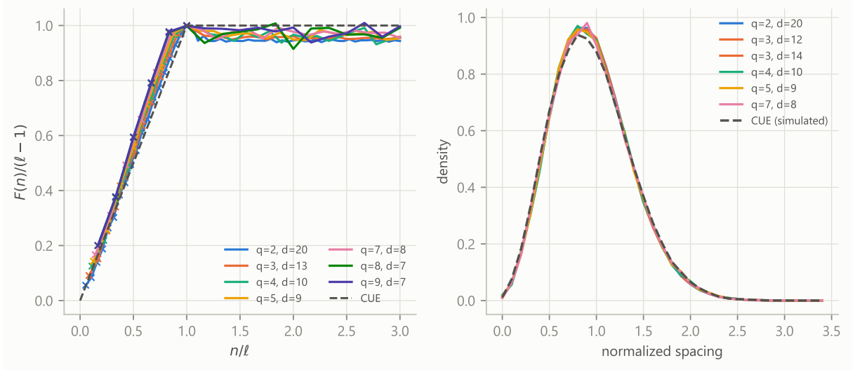
Figure 3: Left: the form factor F(n)/(\ell-1) against n/\ell for several (q, d) , with the CUE value \min(n, \ell-1)/(\ell-1) and the exact diagonal of Proposition 7.1 (crosses). Right: nearest-neighbour spacing densities against CUE.
