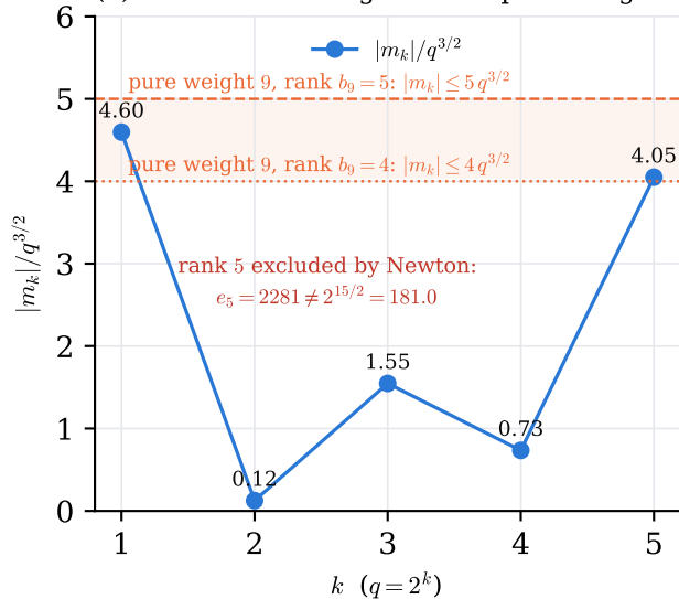
(a) the five values against the pure weight-9 bound
