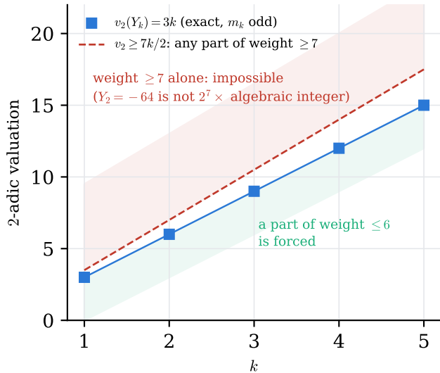
(b) 2-adic constraints under the supersingular
