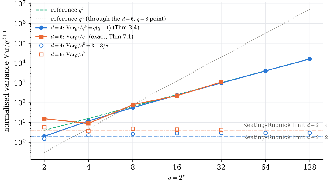
FIGURE 3. Normalised variances against q (log-log). Filled markers: \text{Var}_{\mathcal{G}^2}(\Psi)/q^{d+1} , exact values ( d = 4 : q(q-1) for q \leq 128 , Theorem 3.4; d = 6 : Table 4). Open markers: the full-group variances \text{Var}_{\mathcal{G}}/q^{d+1} , which approach 3 ( d = 4 , Theorem 3.11) and the Keating–Rudnick value 4 ( d = 6 ). The dashed line is q^2 ; the dotted line is a q^4 law normalised through the d = 6 , q = 8 point, which the data exclude. Whether \lim \text{Var}_{\mathcal{G}^2}/q^9 = 1 at d = 6 depends on m_k = o(q^{5/2}) (Theorem 7.1).
