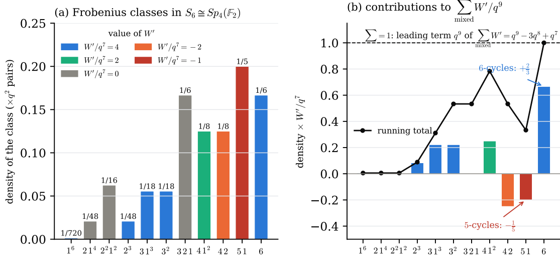
FIGURE 3. The mixed sums W' for odd k by Frobenius class (Table 3), the counterpart of Figure 2. (a) Asymptotic density of each of the eleven classes of S_6 \cong Sp_4(\mathbb{F}_2) among the (q-1)^2 pairs (\lambda_3, \lambda_5) , coloured by the value of W'/q^7 : the 5-cycles ( 1/5 ) carry -q^7 ; the 6-cycles ( 1/6 ), the two classes of order 3 ( 1/18 each), the class 2^3 and the identity carry +4q^7 ; the two classes of order 4 ( 1/8 each) carry \pm 2q^7 and cancel to leading order; the remaining classes vanish. (b) Density times value: the running total reaches exactly 1, the leading coefficient of \sum_{\text{mixed}} W' = q^9 - 3q^8 + q^7 (Proposition 6.18(c)), the negative -q^9/5 of the 5-cycles being overcompensated by the 6-cycles ( +2q^9/3 ) and the order-3 classes ( +4q^9/9 ).
