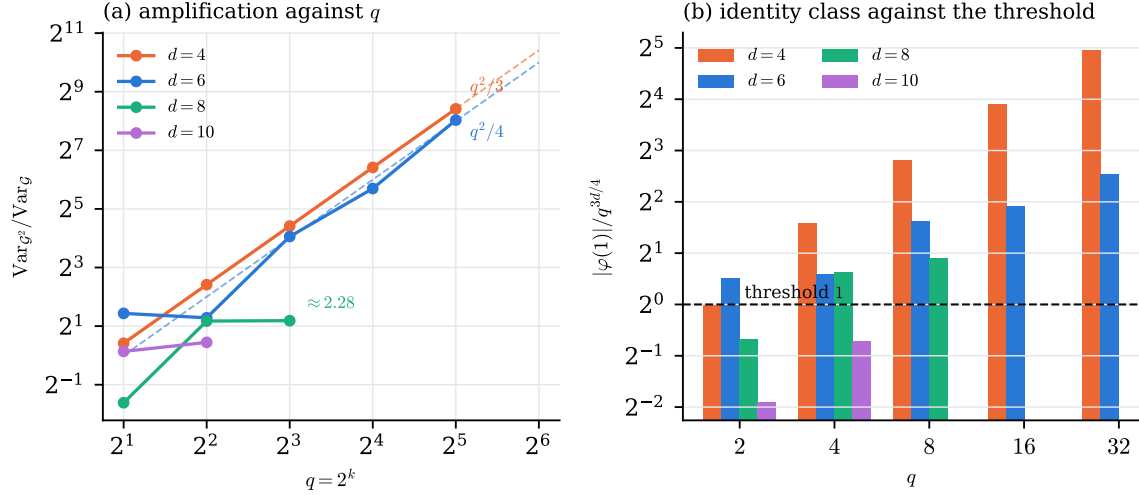
FIGURE 8. The Legendre amplification for even d (data of Table 6). (a) \text{Var}_{\mathcal{G}^2} / \text{Var}_{\mathcal{G}} against q on logarithmic scales: q^2/3 exactly at d = 4 , about q^2/4 at d = 6 , and no growth at d = 8 (2.25, 2.28 at q = 4, 8 ) or d = 10 . (b) The identity-class deviation |\varphi(1)| relative to the threshold q^{3d/4} of Proposition 9.1(c): far above it for d = 4 (where it equals q - 1 ) and d = 6 , at it for d = 8 (1.5, 1.9 at q = 4, 8 ), below it for d = 10 .
