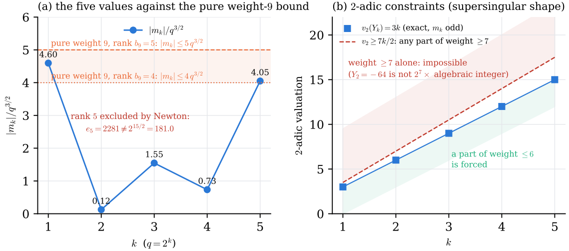
FIGURE 6. What the five values m_k say (Propositions 7.8 and 7.10). (a) |m_k|/q^{3/2} for k \leq 5 against the bound b_9 of a pure weight-9 object of rank b_9 : the value 4.60 at k = 1 forces b_9 \geq 5 , and b_9 = 5 is excluded because the fifth elementary symmetric function of the normalised eigenvalues computed from m_1, \dots, m_5 is 2281 \neq 2^{15/2} . (b) Under the supersingular shape of the eigenvalues, a part of weight \geq 7 has 2-adic valuation \geq 7k/2 , while v_2(Y_k) = 3k exactly ( m_k odd); hence no single weight \geq 7 can carry Y ( Y_2 = -64 ) and a part of weight \leq 6 is forced.
