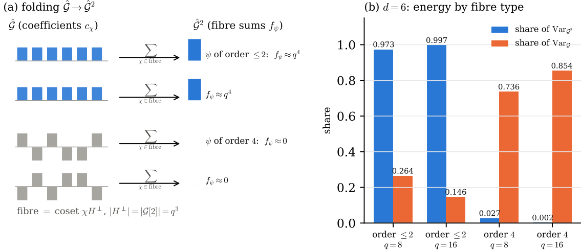
FIGURE 7. Spectral folding at d = 6 . (a) The restriction map \hat{\mathcal{G}} \rightarrow \hat{\mathcal{G}}^2 : each fibre is a coset of H^\perp = \widehat{\mathcal{G}/\mathcal{G}^2} of size |\mathcal{G}[2]| = q^3 , and the fibre sum f_\psi is the \psi -coefficient of \varphi on \mathcal{G}^2 . Over the q characters of \mathcal{G}^2 of order \leq 2 the coefficients add in phase (they are the biased supersingular sums S, S' of Sections 6.6–6.7); over the q^2 - q characters of order 4 they cancel. (b) Shares of \text{Var}_{\mathcal{G}^2} and of \text{Var}_{\mathcal{G}} carried by the two kinds of fibres for q = 8, 16 (Table 5): the coherent fibres hold 97–100% of the Legendre variance but only 15–26% of the full-group energy.
