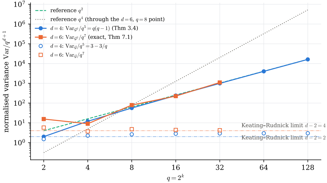
FIGURE 4. Normalised variances against q , both axes logarithmic. Filled markers are \text{Var}_{\mathcal{G}^2}(\Psi)/q^{d+1} , exact values ( d = 4 : q(q-1) for q \leq 128 , Theorem 3.4; d = 6 : Table 4). Open markers: the full-group variances \text{Var}_{\mathcal{G}}/q^{d+1} , which approach 3 ( d = 4 , Theorem 3.11) and the Keating–Rudnick value 4 ( d = 6 ). The dashed line is q^2 ; the dotted line is a q^4 law normalised through the d = 6 , q = 8 point, which the data exclude. Whether \lim \text{Var}_{\mathcal{G}^2}/q^9 = 1 at d = 6 depends on m_k = o(q^{5/2}) (Theorem 7.1).
