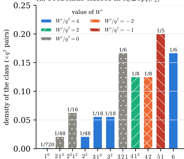
(a) Frobenius classes in S_6 \cong Sp_4(\mathbb{F}_2)
