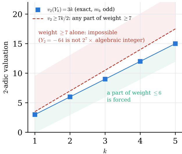
(b) 2-adic constraints (supersingular shape)
