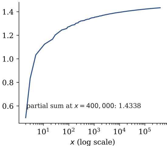
Brun-summable: the sum converges
