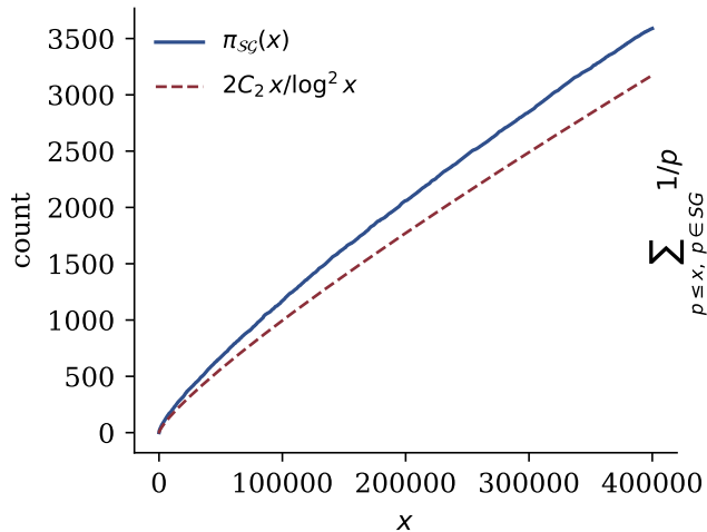
Sophie Germain counting function
