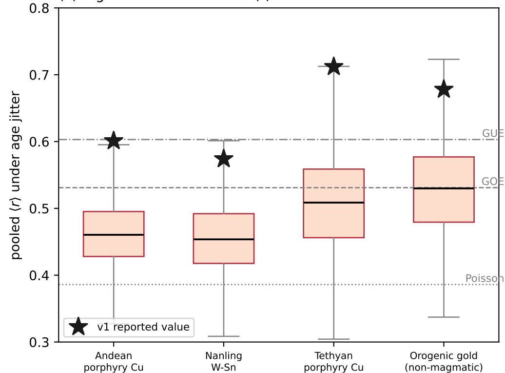
(c) age-error Monte Carlo: \langle r \rangle unresolvable
