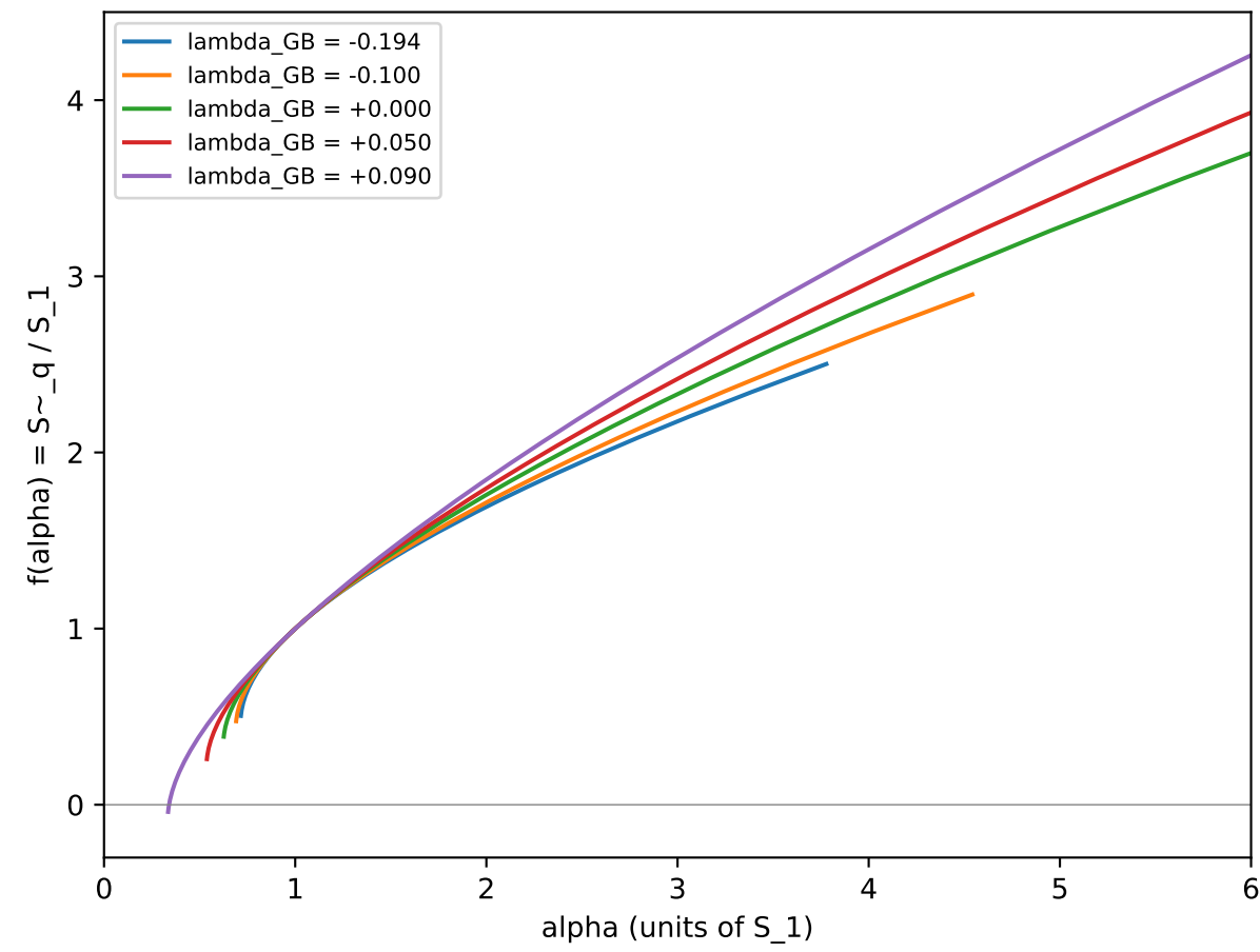
Gauss-Bonnet cosmic branes, d = 4
