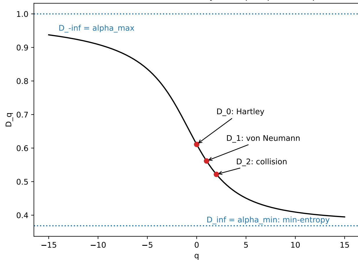
Wave-function multifractality at the quantum Hall transition (participation spectrum of |\psi|^2 , not of \rho_A )
