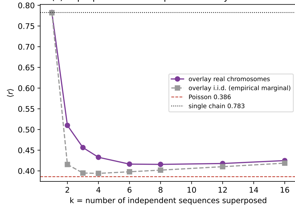
(c) superposition of independent arrays -> Poisson
