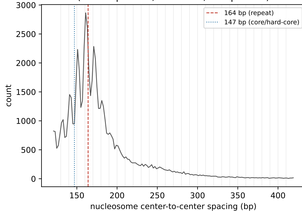
(b) spacing distribution (~164 bp mode, hard core, 10-bp comb)
