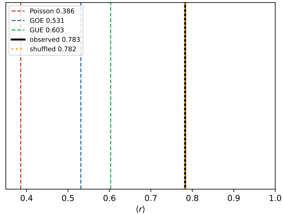
(a) \langle r \rangle : observed = shuffled = scalar/steric, NOT GOE
