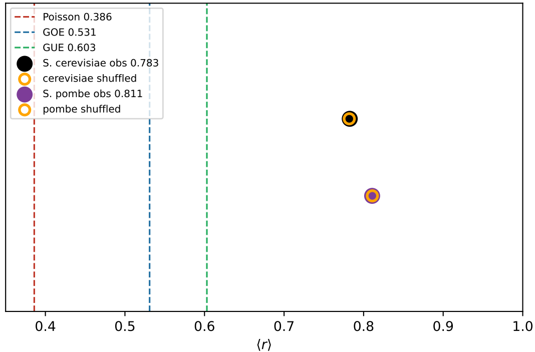
(a) both species: obs = shuffled = scalar, NOT GOE
