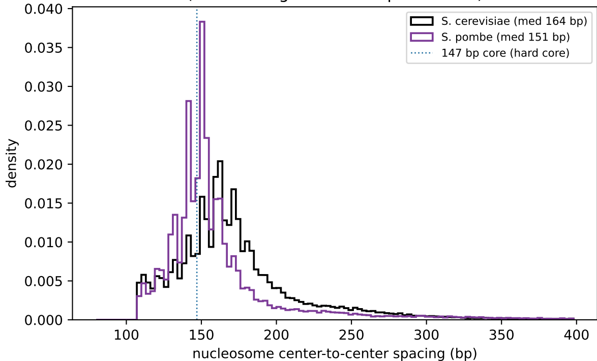
(b) pombe spacing shorter/tighter -> higher \langle r \rangle (scalar marginal tracks species NRL)
